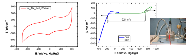
Figure 3: CV of 0,5 mg cm^{-2} La_{0,6}Ca_{0,4}CoO_3 -Vulcan (1:1)/TCP (left) in 6 M KOH / N_2 at 40 mV s^{-1} and (right) in 6M KOH / air at 5 mV s^{-1} and 25^{\circ}C .
