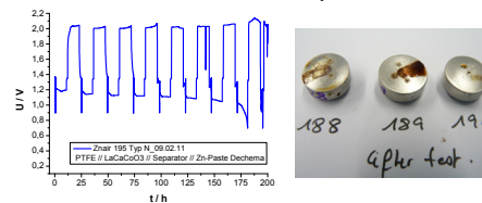
Figure 6: Left: 8 discharge/charge cycles of a button zinc/air cell with a zinc paste, Celgard separator and La_{0,6}Ca_{0,4}CoO_3 /active carbon air electrode. Right: Zn/air cells after test
